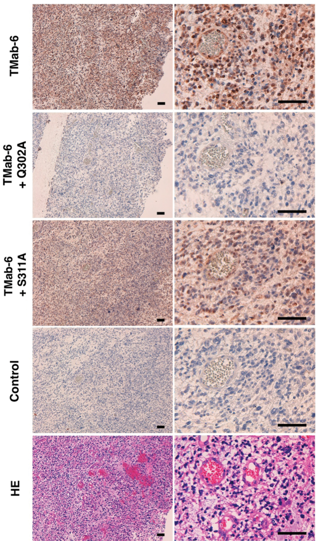
FIG. 1. Immunohistochemistry using TMAb-6 and point mutants of TERT. Glioblastoma tissues were autoclaved in citrate buffer for 20 minutes. Sections were then incubated with TMAb-6, TMAb-6 + Q302A, or TMAb-6 + S311A, and treated using an Envision+ kit. Color development was performed using 3,3-diaminobenzidine tetrahydrochloride. Sections were then counterstained with hematoxylin. Scale bars = 100 μm. HE, hematoxylin and eosin staining; TERT, telomerase reverse transcriptase.
